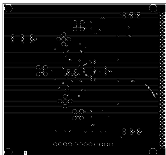
Figure 30. Ground Plane
