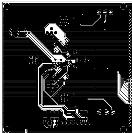
Figure 32. Bottom Routing
