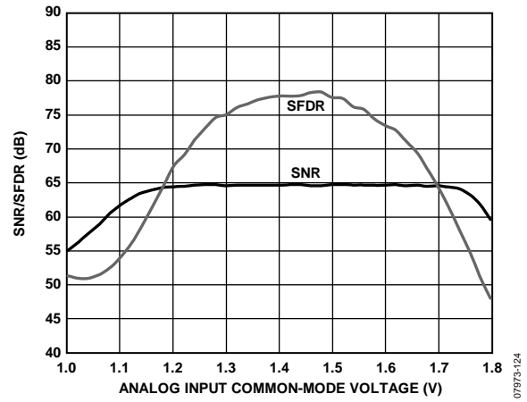
Figure 24. SNR/SFDR vs. Analog Input Common-Mode Voltage, f_{IN} = 84.3 MHz, f_{SAMPLE} = 210 MSPS
