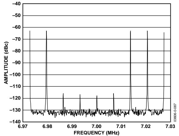
Figure 61. AD9861 Tx Path FFT, In-Band IMD Products of OFDM Signal in Figure 58
