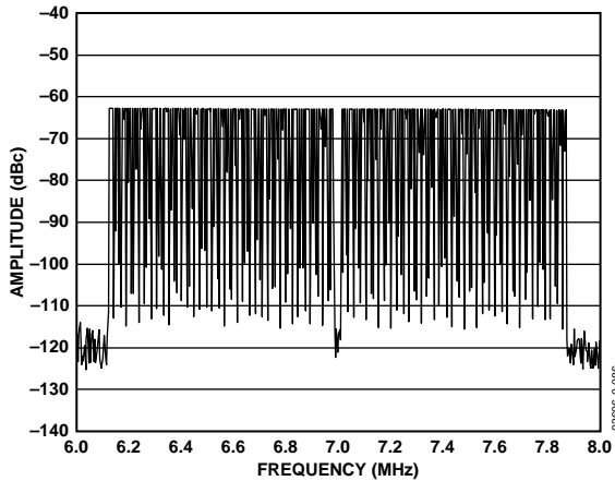
Figure 58. AD9861 Tx Path FFT, 256-Carrier OFDM Signal over 1.75 MHz Bandwidth, Centered at 7 MHz, with 20 mA Full-Scale Output into 60 \Omega Differential Load
