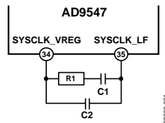
Figure 46. External Loop Filter Schematic
