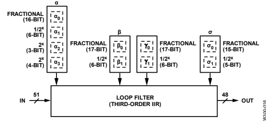
Figure 40. Third-Order Digital IIR Loop Filter
