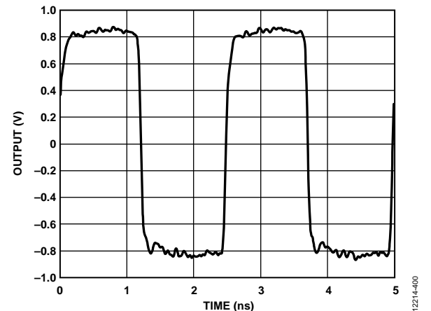
Figure 14. Output Waveform, 28 mA LVPECL-Compatible Mode (400 MHz) with 100Ω Termination Resistor
