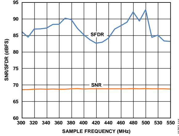
Figure 89. SNR/SFDR vs. f_s , f_{IN} = 170.3 \text{ MHz} ; Buffer Control 1 = 2.0x
