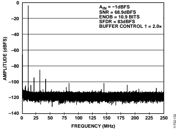
Figure 80. Single-Tone FFT with f_{IN} = 10.3 MHz
