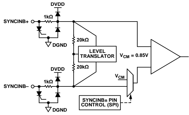
Figure 108. SYNCINB± Inputs
