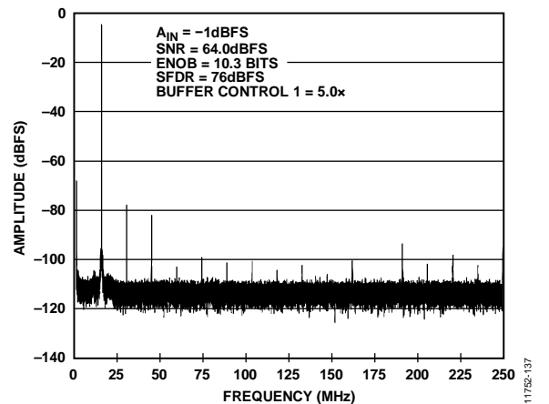
Figure 85. Single-Tone FFT with f_{IN} = 985.3 MHz
