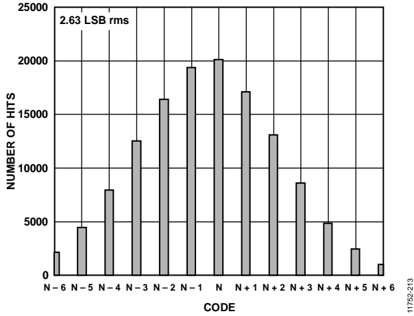
Figure 52. Input-Referred Noise Histogram
