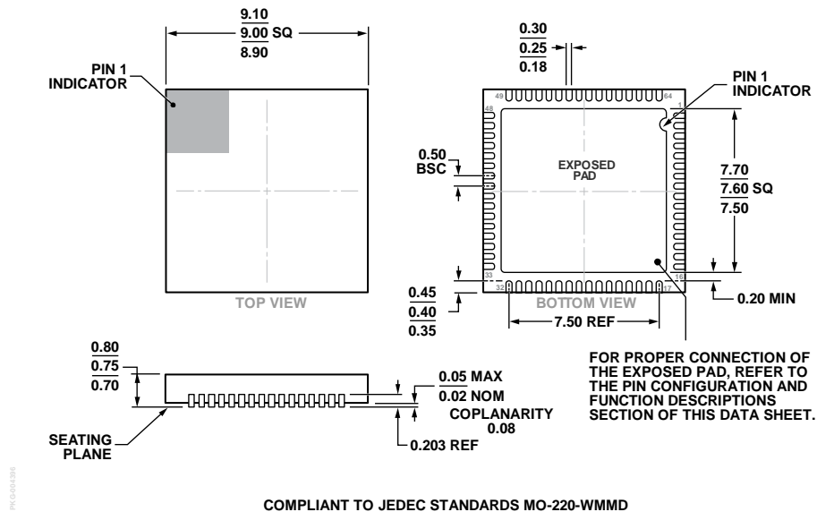
COMPLIANT TO JEDEC STANDARDS MO-220-WMMD Figure 176. 64-Lead Lead Frame Chip Scale Package [LFCSP_WQ] 9 mm x 9 mm Body, Very Thin Quad (CP-64-15) Dimensions shown in millimeters
