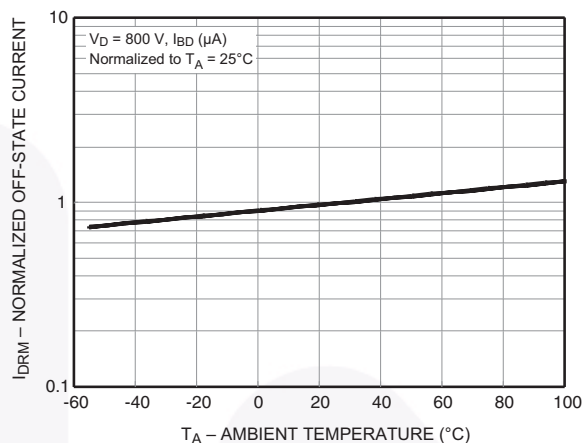
Figure 11. Normalized Off-State Current ( I_{DRM} ) vs. Ambient Temperature ( T_A )
