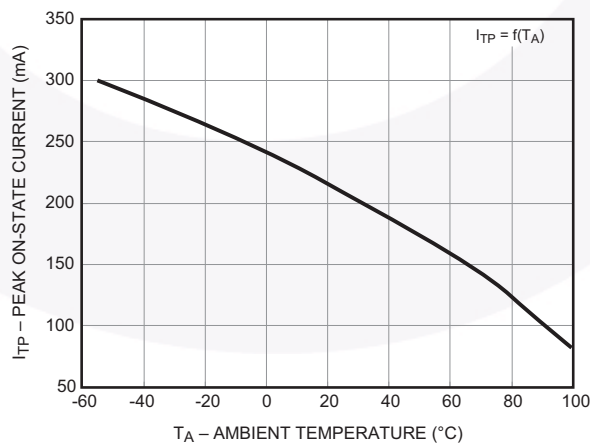
Figure 14. Current Reduction
