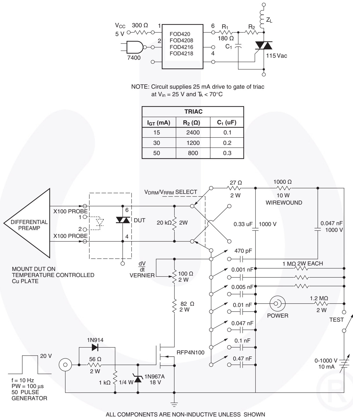
Figure 13. Circuit for Static \frac{dv}{dt} Measurement of Power Thyristors
