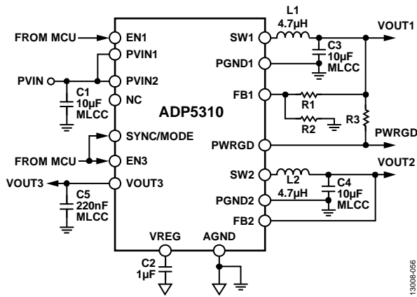
Figure 56. Typical Application Circuit
