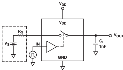
Figure 21. Charge Injection
