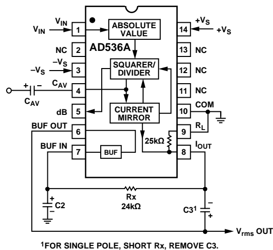
Figure 21. Two-Pole Postfilter
