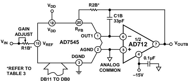
Figure 39. Unipolar Binary Operation
