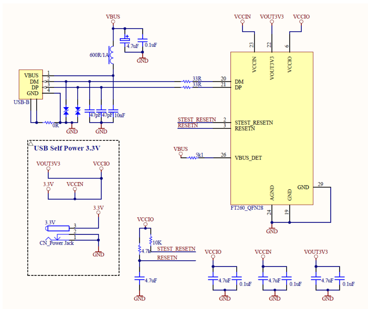
Figure 7.3 Self Powered Configuration with 3.3V Source Input
