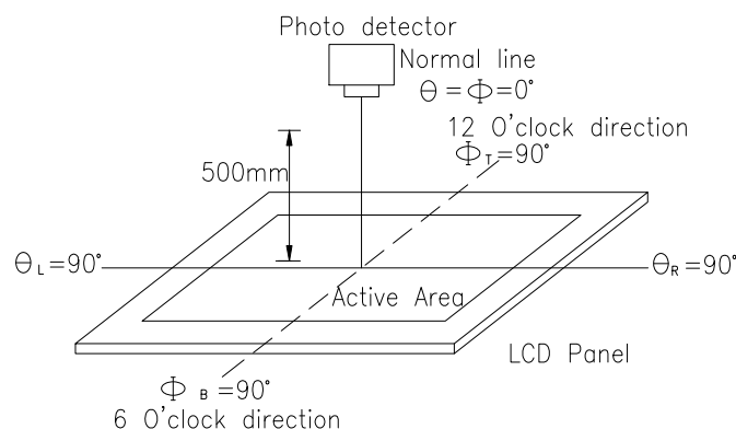
Fig. Optical measurement system setup
