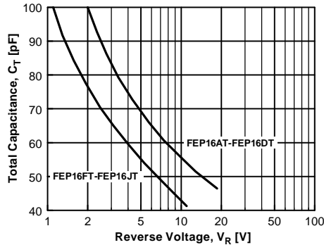
Figure 5. Total Capacitance
