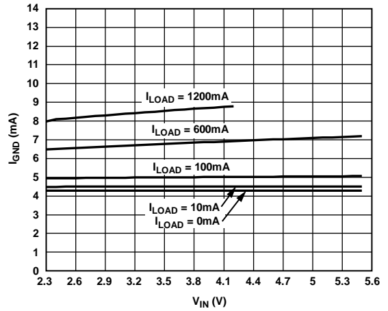
Figure 20. Ground Current ( I_{GND} ) vs. Input Voltage ( V_{IN} ) at Various Loads, V_{OUT} = 1.2 V
