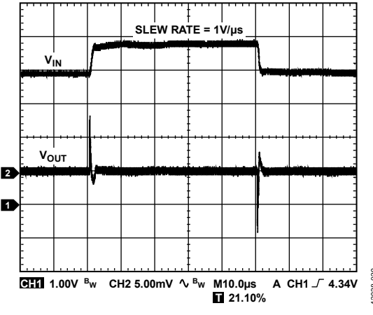
Figure 37. Line Transient Response, 1 \text{ V} Input Step, I_{LOAD} = 1.2 \text{ A} , V_{OUT} = 3.3 \text{ V} , V_{IN} = 3.8 \text{ V} , Channel 1 = V_{IN} , Channel 2 = V_{OUT}
