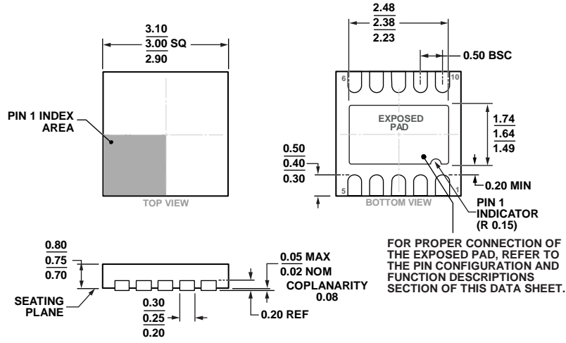
Figure 65. 10-Lead Lead Frame Chip Scale Package [LFCSP] 3 mm x 3 mm Body and 0.75 mm Package Height (CP-10-9) Dimensions shown in millimeters
