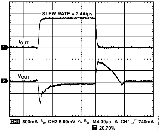
Figure 36. Load Transient Response, I_{LOAD} = 100 \text{ mA} to 1.2 \text{ A} , V_{OUT} = 1.8 \text{ V} , V_{IN} = 2.5 \text{ V} , C_{OUT} = 22 \mu\text{F} , Channel 1 = I_{OUT} , Channel 2 = V_{OUT}
