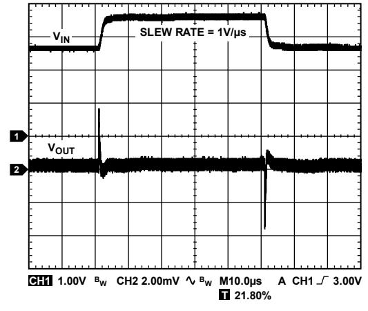
Figure 38. Line Transient Response, 1 \text{ V} Input Step, I_{LOAD} = 1.2 \text{ A} , V_{OUT} = 1.8 \text{ V} , V_{IN} = 2.5 \text{ V} , Channel 1 = V_{IN} , Channel 2 = V_{OUT}
