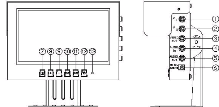
Fig. 2 Connectors and Controls
