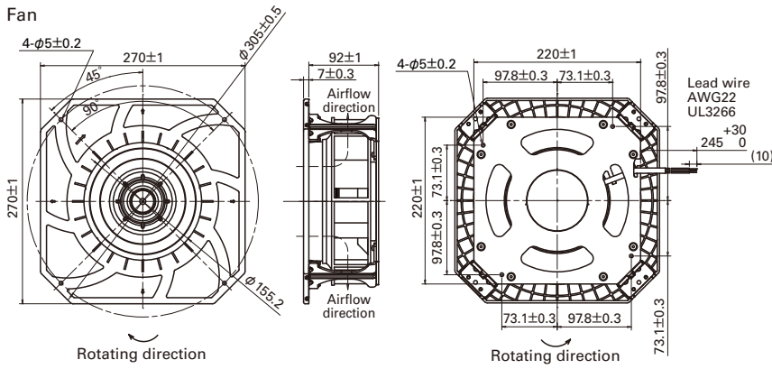
Finger guard (Model: 109-1146)
