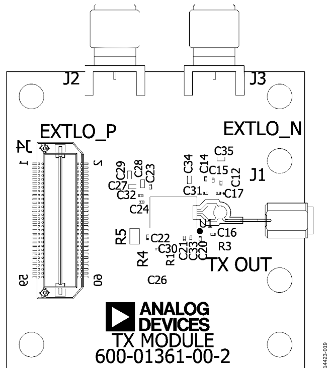
Figure 19. Evaluation PCB Daughter Board
