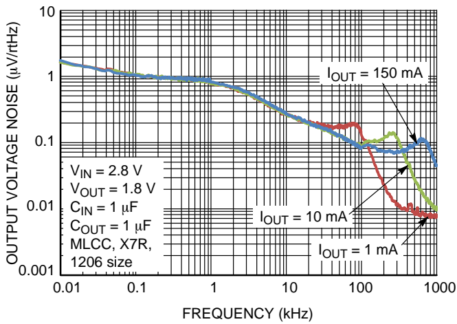
Figure 28. Output Voltage Noise Spectral Density for V OUT = 1.8 V, C OUT = 1 µF
