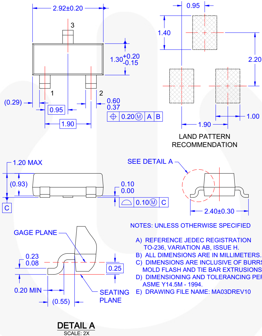
Figure 6. 3-LEAD, SOT23, JEDEC TO-236, LOW PROFILE
