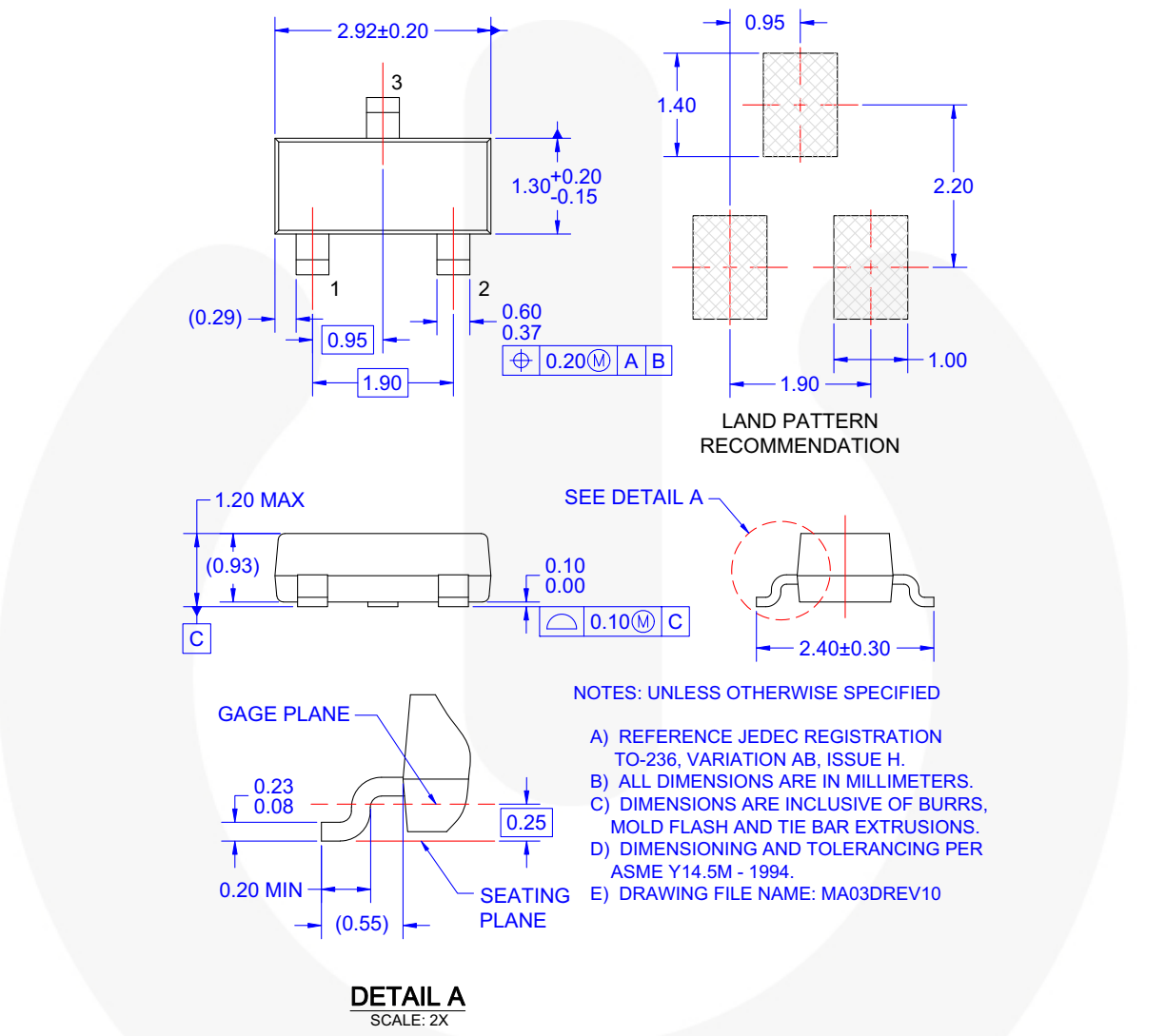
Figure 22. 3-LEAD, SOT-23, JEDEC TO-236, LOW PROFILE
