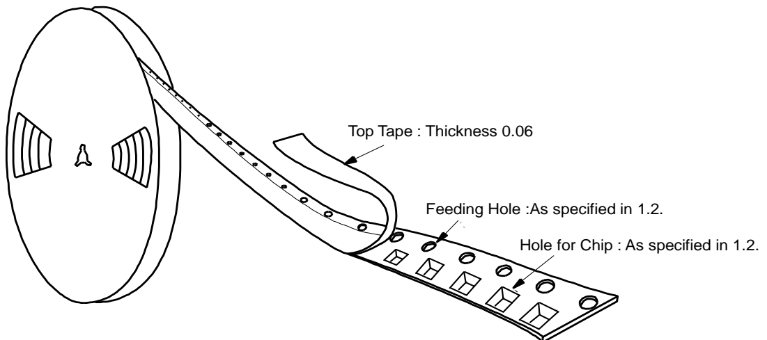
Fig.3 Taping Diagram
