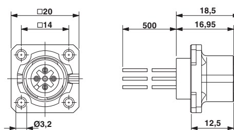
M12 flush-type socket, square flange
