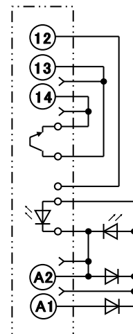
12 V DC Terminal Arrangement/Internal Connections (Top View)
