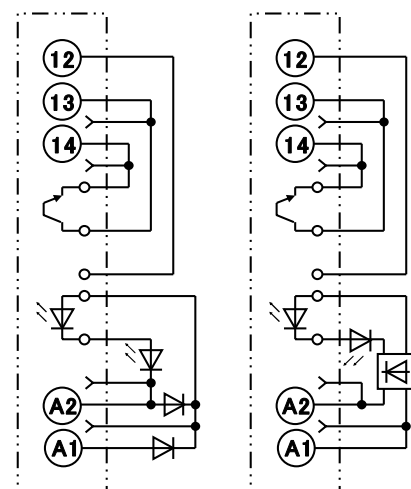
24 V DC Terminal Arrangement/Internal Connections (Top View)
