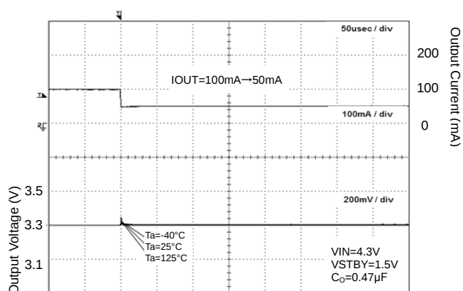
Figure 22. Load Response
