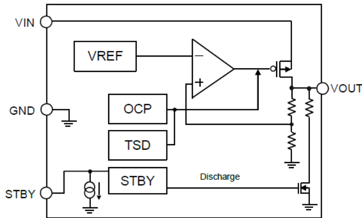
Figure 2. Block Diagram
