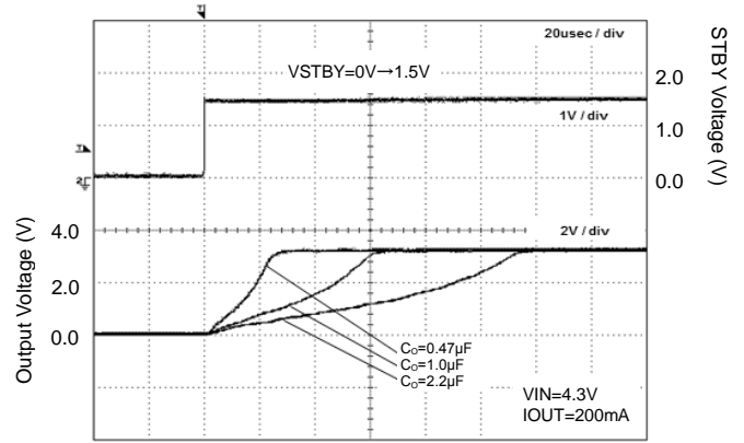
Figure 24. Start Up Time IOUT=200mA
