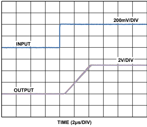
Figure 16. Differential Overload Recovery, Rising
