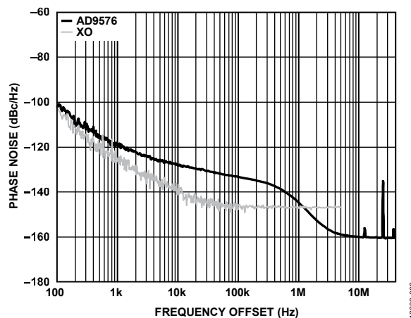
Figure 8. Phase Noise (OUT2)— f_{OUT2} = 156.25\text{ MHz} (HSTL)
