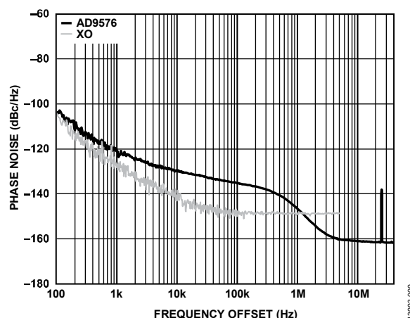
Figure 9. Phase Noise (OUT3)— f_{OUT3} = 125\text{ MHz} (HSTL), f_{OUT4} = 100\text{ MHz} (HSTL)
