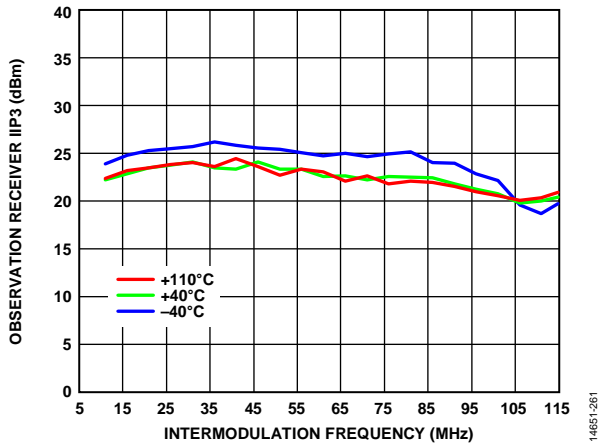
Figure 224. Observation Receiver IIP3 vs. Intermodulation Frequency, 5600 MHz LO, 0 dB Attenuation, 200 MHz RF Bandwidth, 245.76 MSPS Sample Rate
