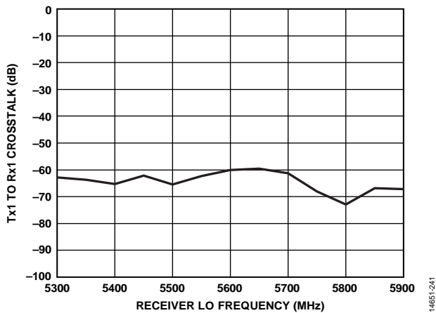
Figure 202. Tx1 to Rx1 Crosstalk vs. Receiver LO Frequency, 100 MHz Receiver RF Bandwidth, 75 MHz Transmitter RF Bandwidth, CW Signal 3 MHz Offset from LO
