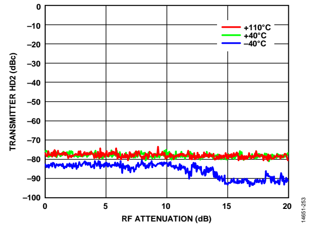
Figure 214. Transmitter HD2 vs. RF Attenuation, 5850 MHz LO, 5855 MHz CW Desired Signal, 75 MHz RF Bandwidth, 245.76 MSPS Sample Rate
