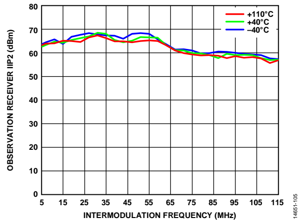
Figure 164. Observation Receiver IIP2 vs. Intermodulation Frequency, 3500 MHz LO, 0 dB Attenuation, 240 MHz RF Bandwidth, 307.2 MSPS Sample Rate
