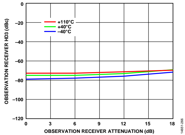
Figure 229. Observation Receiver HD3 vs. Observation Receiver Attenuation, 5600 MHz LO, CW Signal 30 MHz Offset, -15 dBm Input, Input Power Increasing Decibel with Attenuation, 200 MHz RF Bandwidth, 245.76 MSPS Sample Rate
