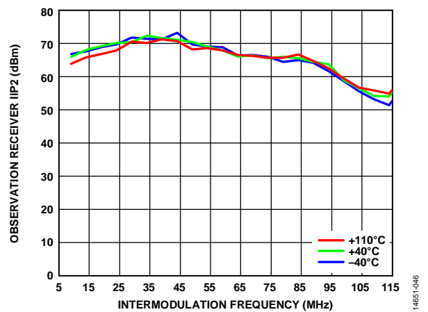
Figure 105. Observation Receiver IIP2 vs. Intermodulation Frequency, 2600 MHz LO, 0 dB Attenuation, 200 MHz RF Bandwidth, 245.76 MSPS Sample Rate
