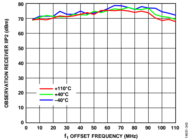
Figure 45. Observation Receiver IIP2 vs. f_1 Offset Frequency, 900 MHz LO, 0 dB Attenuation, 100 MHz RF Bandwidth, f_2 = f_1 + 1 MHz, 122.88 MSPS Sample Rate
