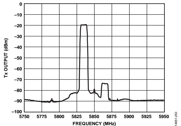
Figure 211. Tx Output Power Spectrum, 3 dB Digital and 1 dB RF Backoff, 40 MHz RF Bandwidth, Transmitter QEC, and Internal LO Leakage Active, LTE 10 MHz Signal, 5850 MHz LO, 1 MHz Resolution Bandwidth, 122.88 MSPS Sample Rate, Test Equipment Noise Floor De-Embedded
