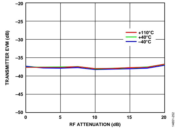
Figure 213. Transmitter EVM vs. RF Attenuation, 5600 MHz LO, Transmitter LO Leakage, and Transmitter QEC Tracking Active, 75 MHz RF Bandwidth, LTE 20 MHz Downlink Signal, 245.76 MSPS Sample Rate
