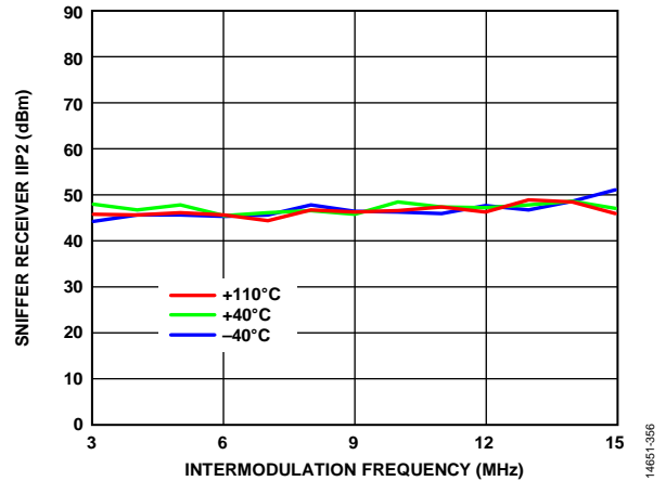
Figure 56. Sniffer Receiver IIP2 vs. Intermodulation Frequency, 600 MHz LO, 0 dB Attenuation, 20 MHz RF Bandwidth, 30.72 MSPS Sample Rate
