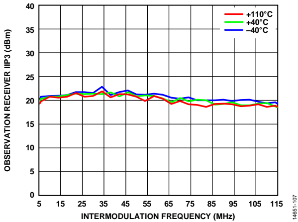
Figure 166. Observation Receiver IIP3 vs. Intermodulation Frequency, 3500 MHz LO, 0 dB Attenuation, 240 MHz RF Bandwidth, 307.2 MSPS Sample Rate
