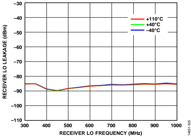
Figure 5. Receiver Local Oscillator (LO) Leakage vs. Receiver LO Frequency, 0 dB Receiver Attenuation, 20 MHz RF Bandwidth, 30.72 MSPS Sample Rate
