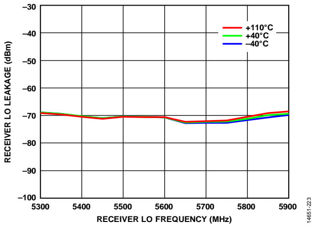
Figure 182. Receiver Local Oscillator (LO) Leakage vs. Receiver LO Frequency, 0 dB Receiver Attenuation, 100 MHz RF Bandwidth, 122.88 MSPS Sample Rate
