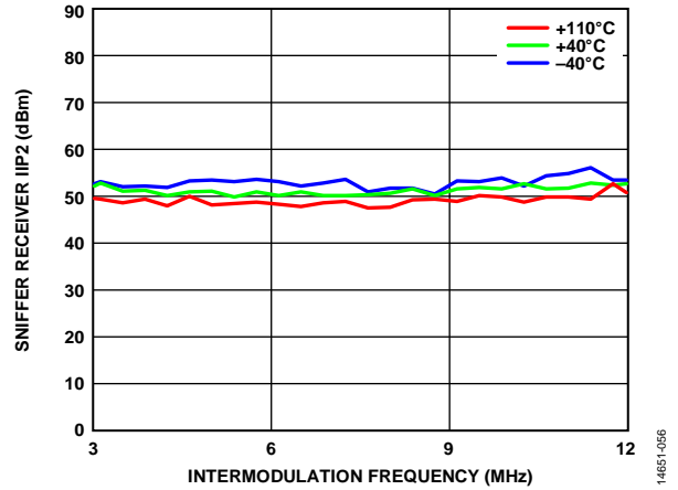
Figure 115. Sniffer Receiver IIP2 vs. Intermodulation Frequency, 2600 MHz LO, 0 dB Attenuation, 20 MHz RF Bandwidth, 30.72 MSPS Sample Rate
