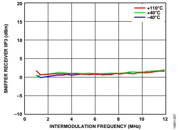
Figure 116. Sniffer Receiver IIP3 vs. Intermodulation Frequency, 2600 MHz LO, 0 dB Attenuation, 20 MHz RF Bandwidth, 30.72 MSPS Sample Rate
