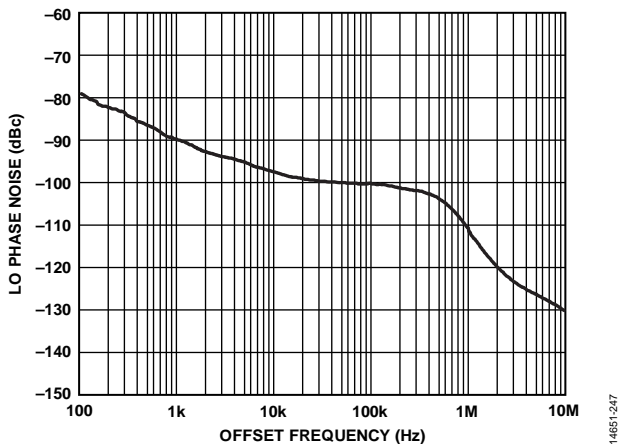
Figure 208. LO Phase Noise vs. Offset Frequency, 3 dB Digital Backoff, 5850 MHz LO
