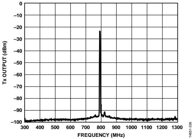
Figure 36. Tx Output Power Spectrum, 2 dB Digital and 3 dB RF Backoff, 20 MHz RF Bandwidth, Transmitter QEC, and Internal LO Leakage Active, LTE 10 MHz Signal, 800 MHz LO, 1 MHz Resolution Bandwidth, 122.88 MSPS Sample Rate, Test Equipment Noise Floor De-Embedded
