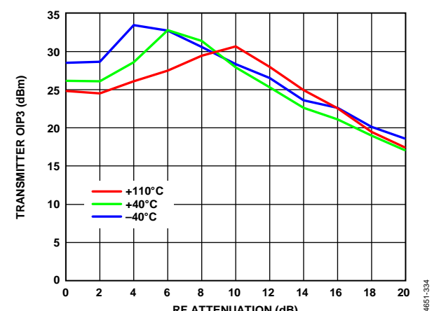
Figure 34. Transmitter OIP3 vs. RF Attenuation, 800 MHz LO, 20 MHz RF Bandwidth, f_1 = 10 MHz, f_2 = 11 MHz, 3 dB Digital Backoff, 122.88 MSPS Sample Rate
