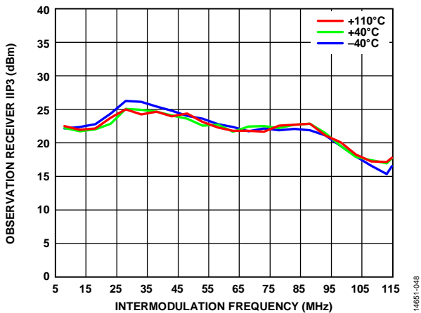
Figure 107. Observation Receiver IIP3 vs. Intermodulation Frequency, 2600 MHz LO, 0 dB Attenuation, 200 MHz RF Bandwidth, 245.76 MSPS Sample Rate
