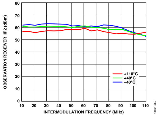
Figure 222. Observation Receiver IIP2 vs. Intermodulation Frequency, 5600 MHz LO, 0 dB Attenuation, 200 MHz RF Bandwidth, 245.76 MSPS Sample Rate
