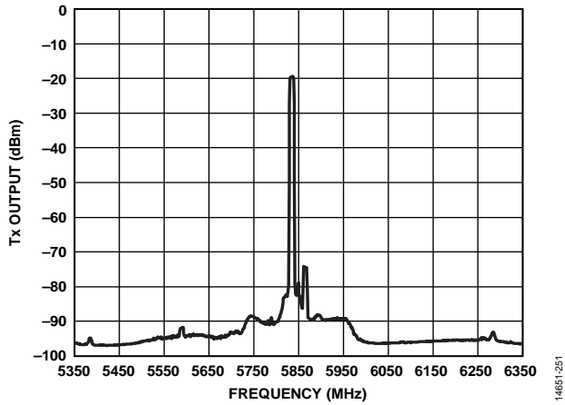
Figure 212. Tx Output Power Spectrum, 3 dB Digital and 1 dB RF Backoff, 40 MHz RF Bandwidth, Transmitter QEC, and Internal LO Leakage Active, LTE 10 MHz Signal, 5850 MHz LO, 1 MHz Resolution Bandwidth, 122.88 MSPS Sample Rate, Test Equipment Noise Floor De-Embedded
