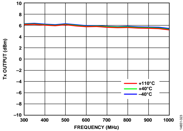
Figure 23. Tx Output Power, Transmitter QEC, and External LO Leakage Tracking Active, 10 MHz CW Offset Signal, 1 MHz Resolution Bandwidth, 122.88 MSPS Sample Rate
