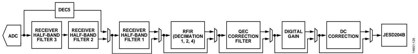
Figure 231. Data Rx Data Path Filter Implementation
