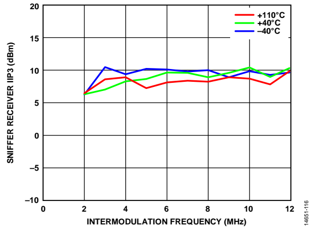
Figure 175. Sniffer Receiver IP3 vs. Intermodulation Frequency, 3500 MHz LO, 0 dB Attenuation, 20 MHz RF Bandwidth, 38.4 MSPS Sample Rate
