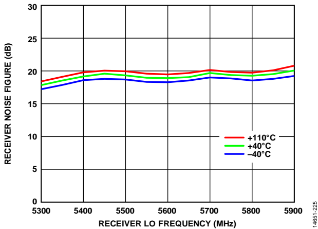
Figure 184. Receiver Noise Figure vs. Receiver LO Frequency, 0 dB Receiver Attenuation, 100 MHz RF Bandwidth, 122.88 MSPS Sample Rate, 50 MHz Integration Bandwidth (Includes 1.2 dB Matching Circuit Loss)
