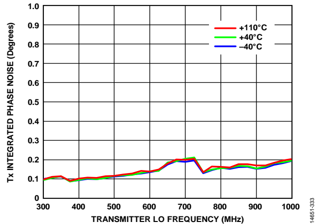
Figure 33. Tx Integrated Phase Noise vs. Transmitter LO Frequency, 20 MHz RF Bandwidth, CW 20 MHz Offset from LO, 3 dB Digital Backoff
