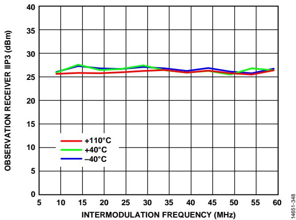
Figure 48. Observation Receiver IIP3 vs. Intermodulation Frequency, 900 MHz LO, 0 dB Attenuation, 100 MHz RF Bandwidth, 122.88 MSPS Sample Rate
