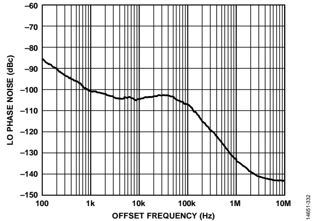
Figure 32. LO Phase Noise vs. Offset Frequency, 3 dB Digital Backoff, 710 MHz LO
