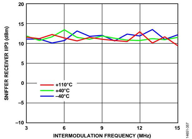
Figure 57. Sniffer Receiver IIP3 vs. Intermodulation Frequency, 600 MHz LO, 0 dB Attenuation, 20 MHz RF Bandwidth, 30.72 MSPS Sample Rate
