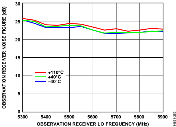
Figure 220. Observation Receiver Noise Figure vs. Observation Receiver LO Frequency, 0 dB Receiver Attenuation, 200 MHz RF Bandwidth, 245.76 MSPS Sample Rate, 100 MHz Integration Bandwidth
