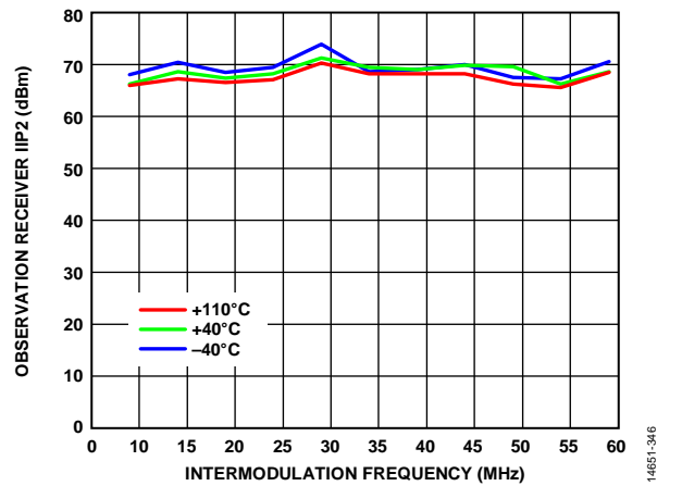
Figure 46. Observation Receiver IIP2 vs. Intermodulation Frequency, 900 MHz LO, 0 dB Attenuation, 100 MHz RF Bandwidth, 122.88 MSPS Sample Rate
