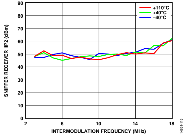
Figure 174. Sniffer Receiver IP2 vs. Intermodulation Frequency, 3500 MHz LO, 0 dB Attenuation, 20 MHz RF Bandwidth, 38.4 MSPS Sample Rate
