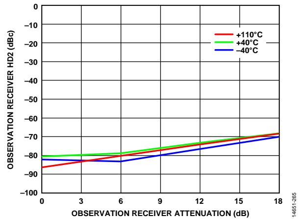
Figure 228. Observation Receiver HD2 vs. Observation Receiver Attenuation, 5600 MHz LO, CW Signal 30 MHz Offset, -15 dBm Input, Input Power Increasing Decibel with Attenuation, 200 MHz RF Bandwidth, 245.76 MSPS Sample Rate
