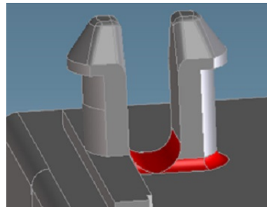
New product with radius (shown in red)
