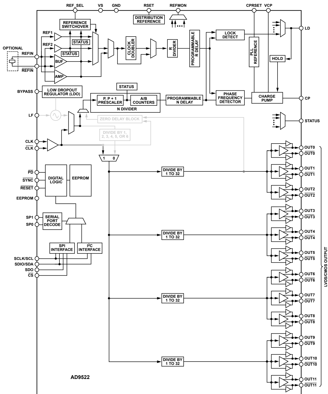
Figure 37. Clock Distribution or External VCO < 1600 MHz (Mode 1)
