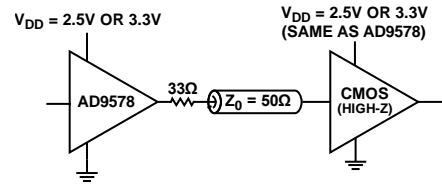
Figure 30. DC-Coupled LVCMOS Termination
