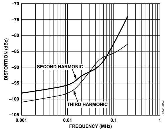
Figure 23. Distortion vs. Frequency, V_S = \pm 12V , R_L = 600\Omega , V_{OUT} = 20V_{p-p}
