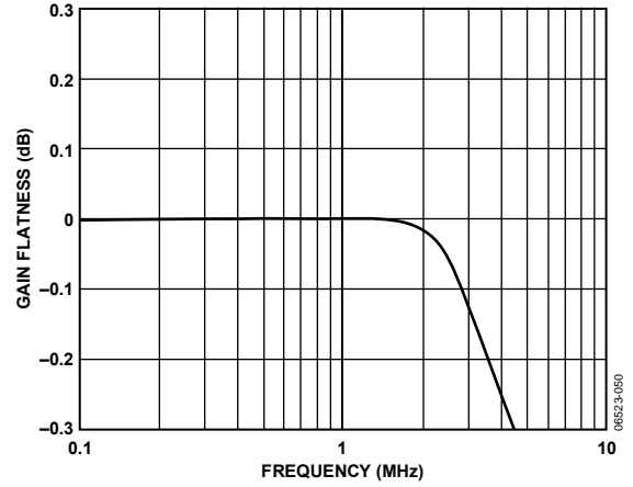
Figure 21. Large-Signal Gain Flatness, V_S = \pm 12V , R_L = 600\Omega , V_{OUT} = 8V_{p-p}
