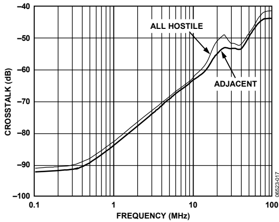
Figure 19. Crosstalk vs. Frequency, V_S = \pm 5V , R_L = 150\Omega , V_{OUT} = 2V_{p-p}
