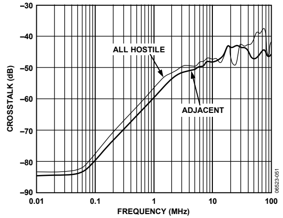
Figure 22. Crosstalk vs. Frequency, V_S = \pm 12V , R_L = 600\Omega , V_{OUT} = 20V_{p-p}
