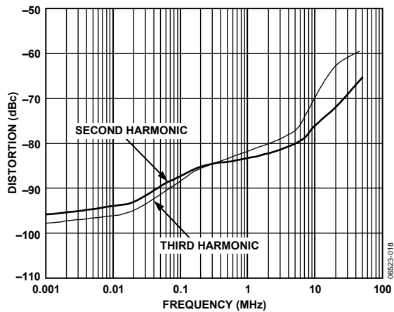
Figure 20. Distortion vs. Frequency, V_S = \pm 5V , R_L = 150\Omega , V_{OUT} = 2V_{p-p}
