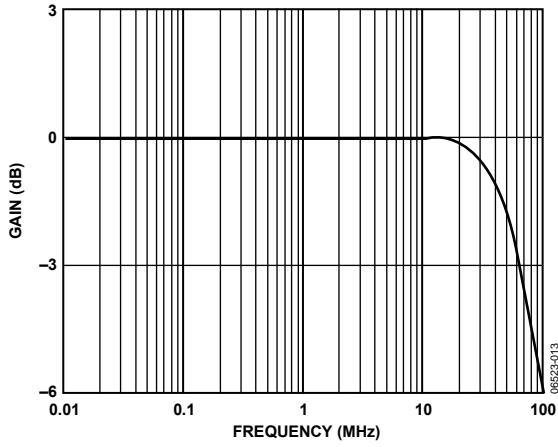
Figure 12. Small-Signal Bandwidth, V_S = \pm 5\text{ V} , R_L = 150\ \Omega , V_{OUT} = 200\text{ mV p-p}
