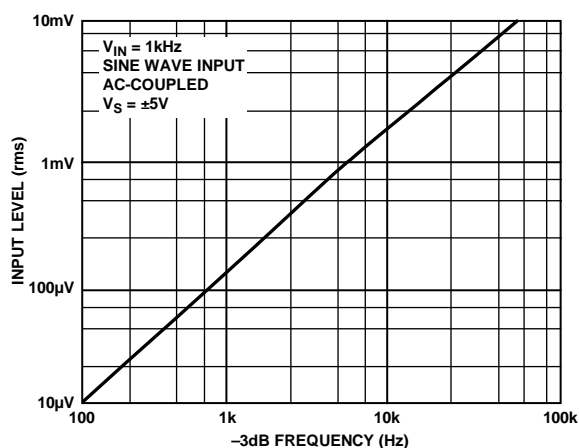
Figure 11. RMS Input Level (Pin 2) vs. -3 dB Frequency
