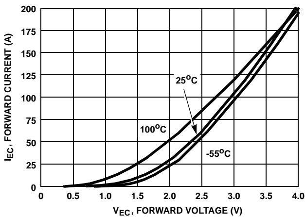
FIGURE 17. DIODE FORWARD CURRENT vs FORWARD VOLTAGE DROP
