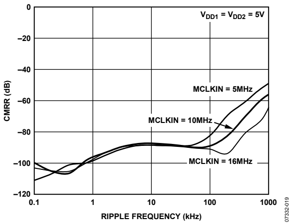
Figure 19. CMRR vs. Common-Mode Ripple Frequency
