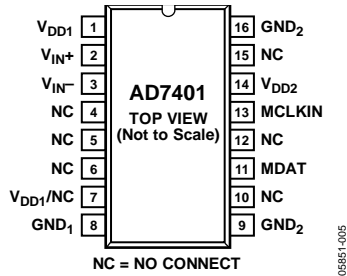
Figure 5. Pin Configuration
