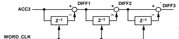
Figure 27. Differentiator
