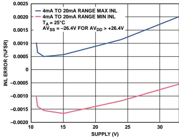
Figure 42. Integral Nonlinearity Error vs. AV_{DD}/|AV_{SS}| , Over Supply, External R_{SET}
