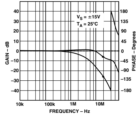
TPC 3. Closed-Loop Gain and Phase, A_V = +1
