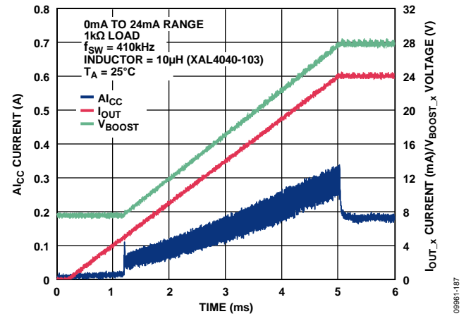
Figure 83. I_{CC} Current vs. Time for 24 mA Step Through 1 k \Omega Load with Slew Rate Control
