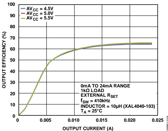
Figure 56. Output Efficiency vs. Output Current (See Figure 78)
