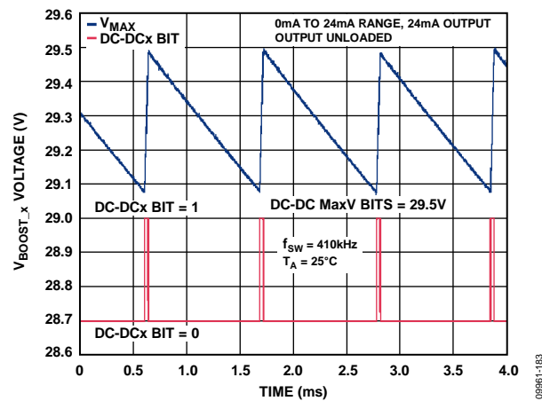
Figure 79. Operation on Reaching V_{\text{MAX}}
