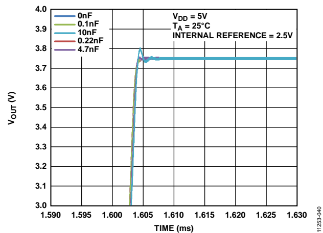
Figure 38. Settling Time vs. Capacitive Load
