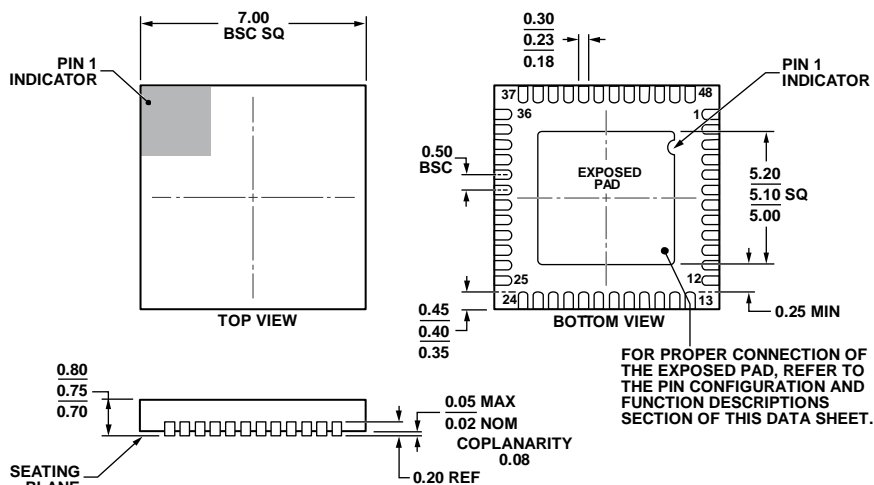
Figure 40. 48-Lead Lead Frame Chip Scale Package [LFCSP] 7 mm × 7 mm Body and 0.75 mm Package Height (CP-48-4)
