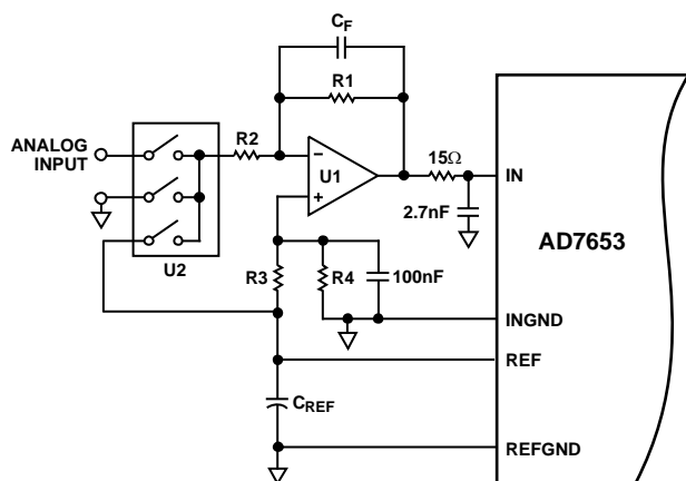
Figure 38. Using the AD7653 in 16-Bit Bipolar and/or Wider Input Ranges
