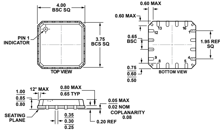
Figure 72. 16-Lead Lead Frame Chip Scale Package [LFCSP_VQ] 4 mm x 4 mm Body, Very Thin Quad, with Hidden Paddle (CP-16-19) Dimensions shown in millimeters
