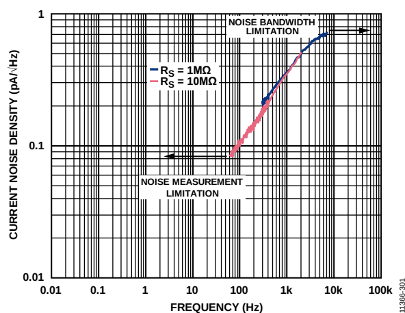
Figure 90. Current Noise Density vs. Frequency
