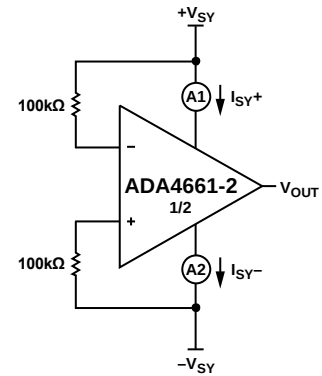
Figure 75. Comparator A
