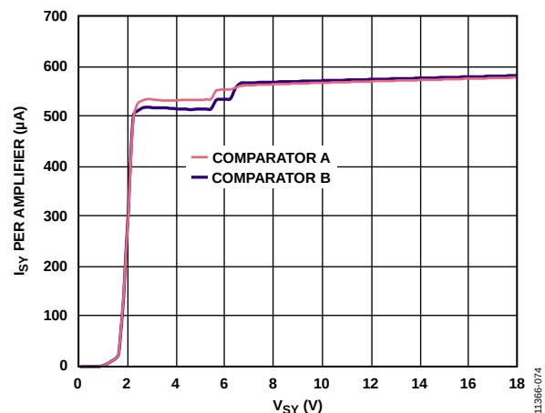
Figure 77. Supply Current vs. Supply Voltage (ADA4661-2 as a Comparator)
