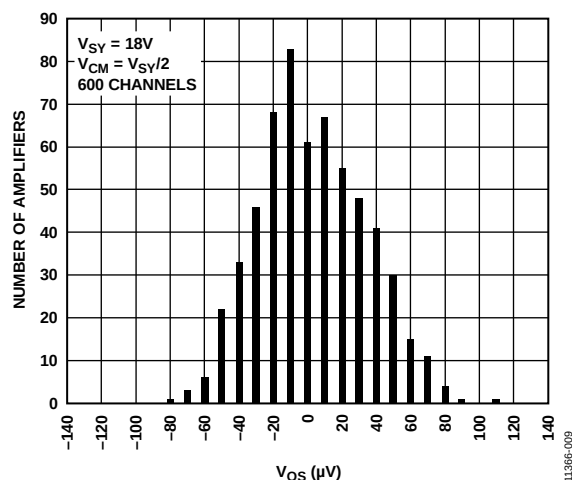
Figure 9. Input Offset Voltage Distribution
