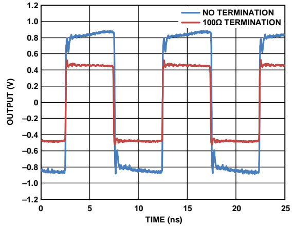
Figure 18. Output Waveform, 14 mA Mode (100 MHz)
