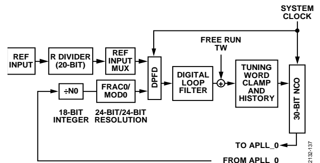
Figure 31. DPLL_0 Core
