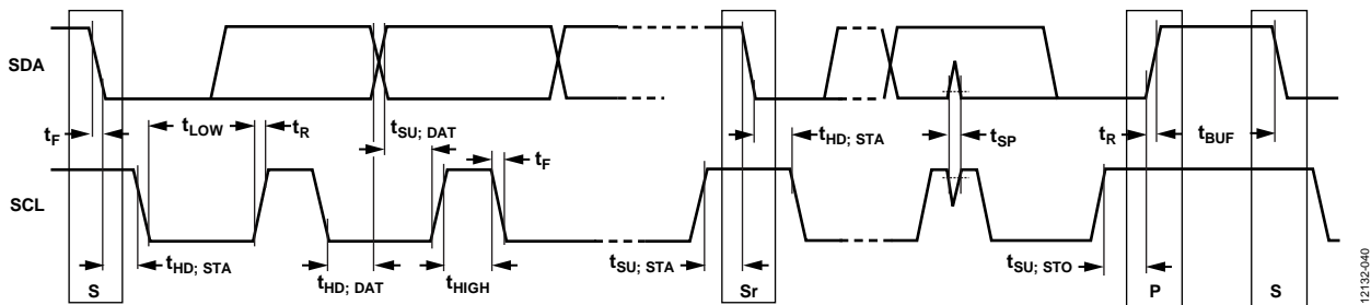
Figure 48. I 2 C Serial Port Timing
