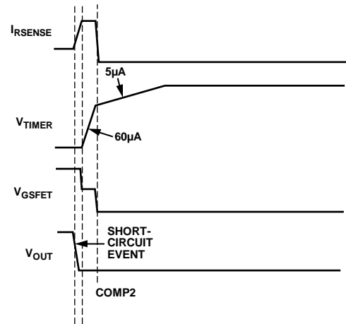
Figure 36. ADM1170-2 Latch Off After Overcurrent Fault
