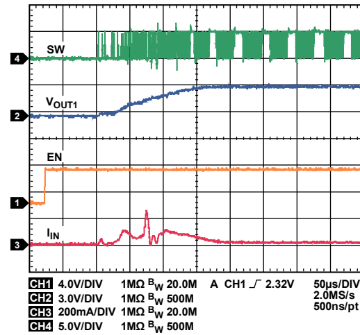
Figure 6. Buck Startup, V_{OUT1} = 3.3\text{ V} , I_{OUT} = 20\text{ mA}
