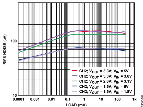
Figure 90. LDO1 Output Noise vs. Load Current, Across Input and Output Voltage
