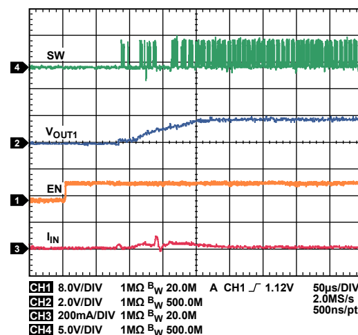
Figure 7. Buck Startup, V_{OUT1} = 1.8\text{ V} , I_{OUT} = 20\text{ mA}
