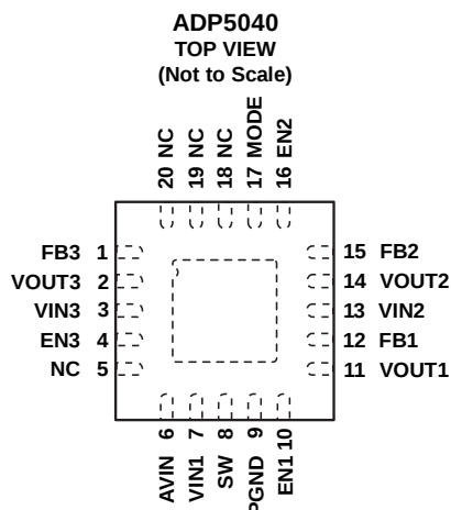
Figure 2. Pin Configuration—View from Top of the Die
