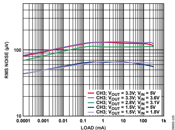
Figure 91. LDO2 Output Noise vs. Load Current, Across Input and Output Voltage
