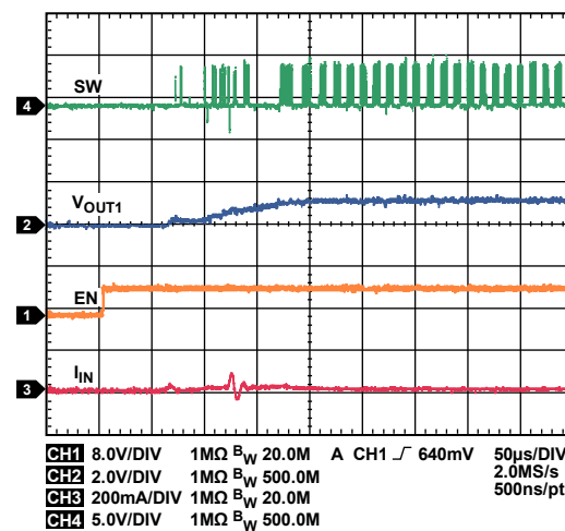
Figure 8. Buck Startup, V_{OUT1} = 1.2\text{ V} , I_{OUT} = 20\text{ mA}
