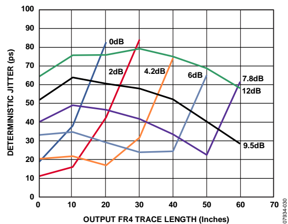
Figure 30. Deterministic Jitter vs. Output FR4 Channel Length
