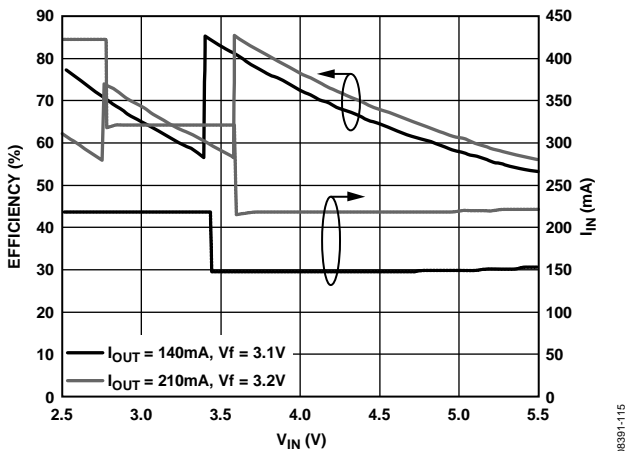
Figure 19. Typical Efficiency (Low Vf Diode)
