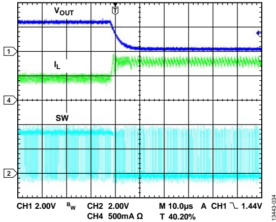
Figure 34. Output Short
